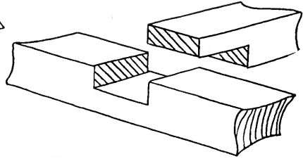
MIDDLE LAP JOINT
